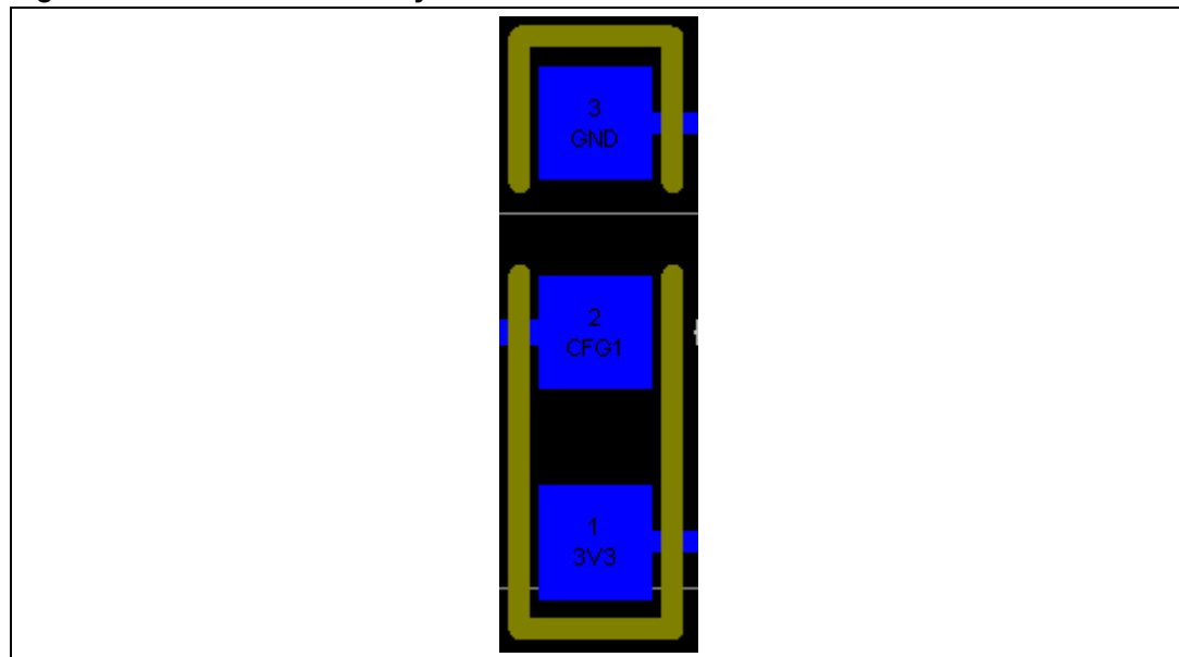
Figure 9. Resistor assembly
